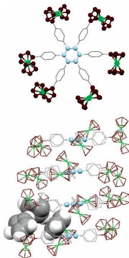
Figure 1. (Top) X-ray structure of 5 showing the varied orientations of the ferrocenyl groups. (Bottom) Packing of 5 in the crystal due to effective CH– \pi interactions that are exemplified by the partial space-filling representations of three cyclopentadienyl moieties from two different molecules.
