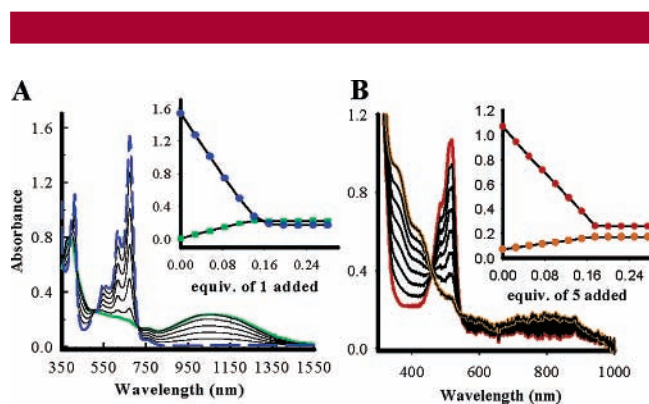
Figure 4. (A) Spectral changes attendant upon the reduction of 1.7 \times 10^{-4} M NAP + ·SbCl 6 - (blue) by incremental addition of 1.2 \times 10^{-3} M 1 to its hexacation radical 1 6+ (green) in CH 2 Cl 2 at 22 °C. Inset. A plot of depletion of absorbance of NAP + (blue circles, at 672 nm) and an increase of the absorbance of 1 6+ (green squares, at 1100 nm) against the equivalent of added 1 . (B) Spectral changes attendant upon the reduction of 1.3 \times 10^{-4} M MA + ·BF 4 - (red) by incremental addition of 1.3 \times 10^{-3} M 5 to its hexacation 5 6+ (yellow-orange) in CH 2 Cl 2 at 22 °C. Inset: plot of depletion of absorbance of MA + (red circles, at 518 nm) and an increase of the absorbance of 5 6+ (orange circles, at 800 nm) against the equivalent of added 5 .
