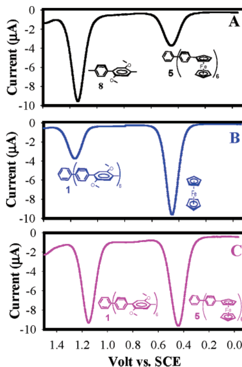
Figure 3. Square-wave voltammograms of mixtures of 0.25 mM 5 and 1.5 mM 8 (A), 0.25 mM 1 and 1.5 mM ferrocene (B), and 0.25 mM each of 1 and 5 (C) in CH 2 Cl 2 containing 0.2 M n -Bu 4 NPF 6 at 22 °C.
